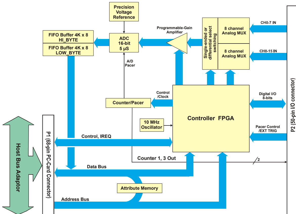
Figure 1. PC-CARD-DAS16/16 functional block diagram
