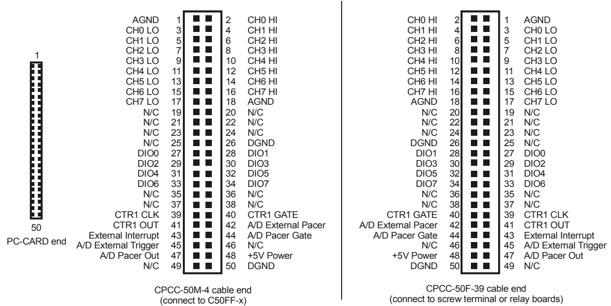
Figure 4. Differential mode cable map — PC-CARD to CPCC-50M-4 and to CPCC-50F-39
