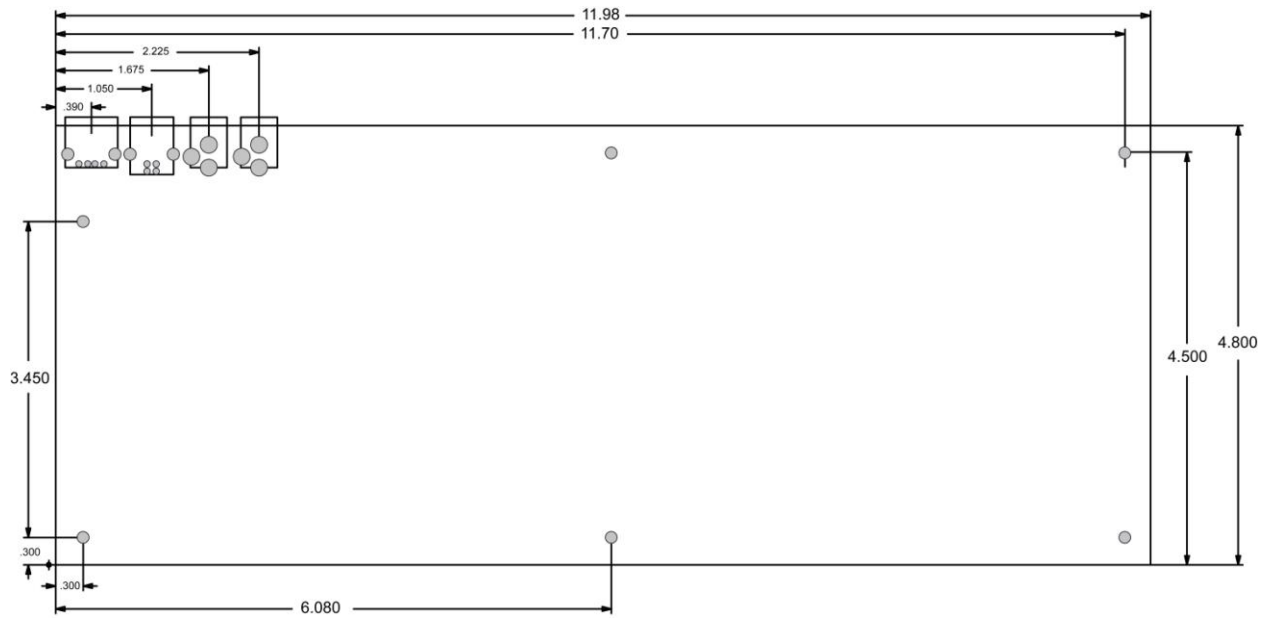
Circuit board dimensions
