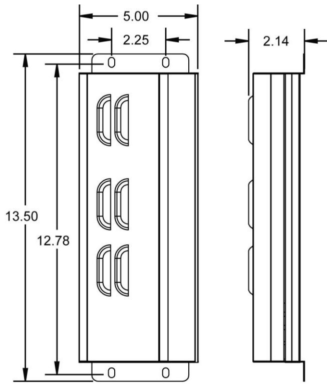
Enclosure dimensions
