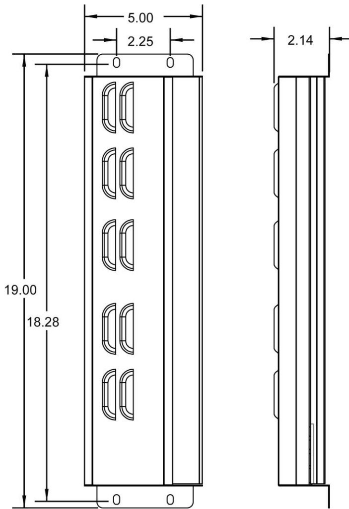
Enclosure dimensions
