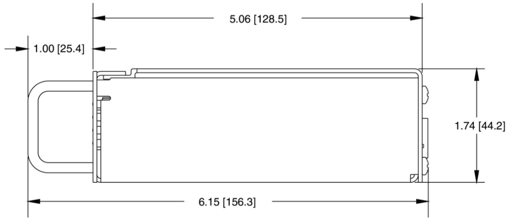
Enclosure dimensions – side
