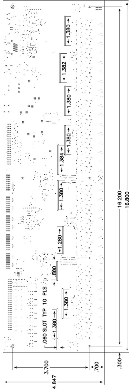
Circuit board dimensions
