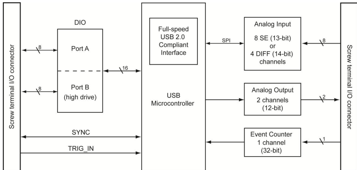
Figure 1. USB-1408FS-Plus functional block diagram
