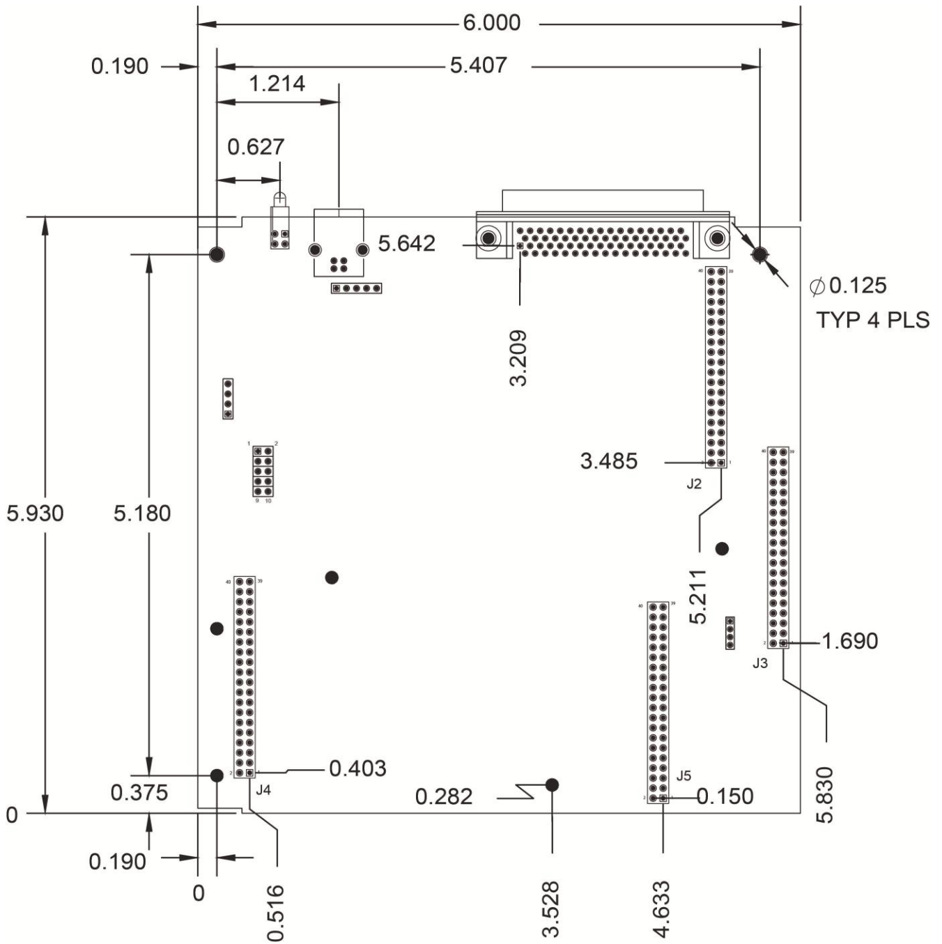
USB-2600 Series Circuit Board
