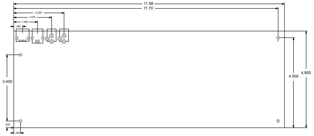
Circuit board dimensions
