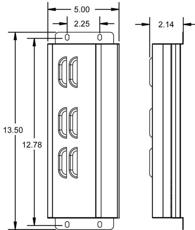
Enclosure dimensions
