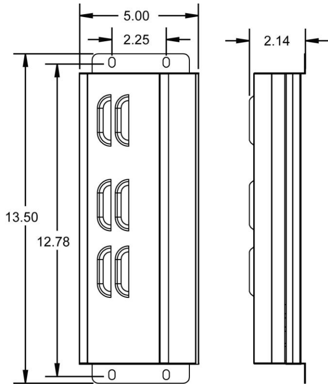
Enclosure dimensions
