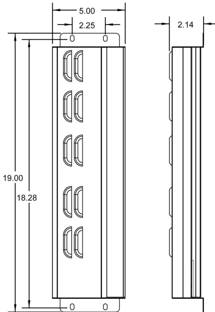
Enclosure dimensions
