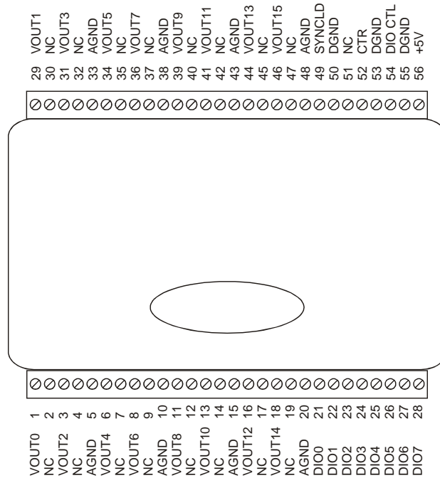
Figure 5. USB-3105 signal pin out
