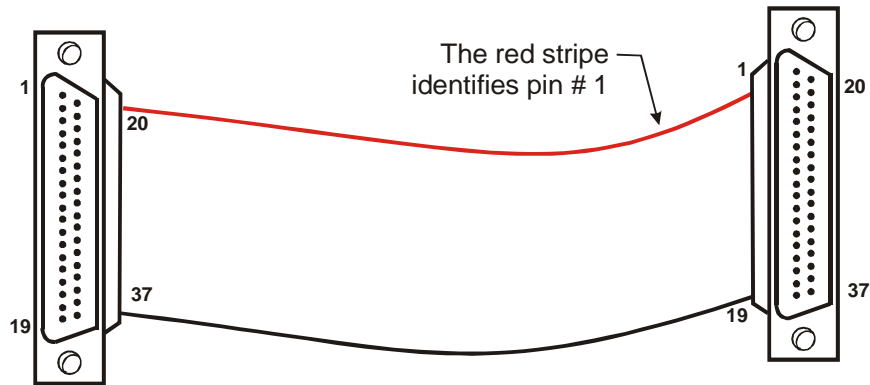
Figure 2. C37FF-x cable
